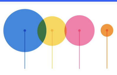
Circles 2 - 4 terms
